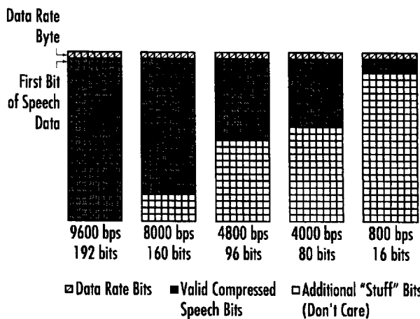
Figure 12. Q4401 Tx and Rx Frame Data Bit Definition
